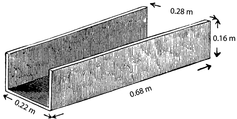
Fig. 6. Terracotta drainage channel found in Room X, a light well (after Schliemann 1976, fig. 118).
