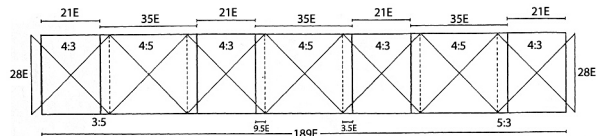
Fig. 2. Layout of the seven units of the Tiryns dado (after Moser v. Filseck 1986, fig. 9).
