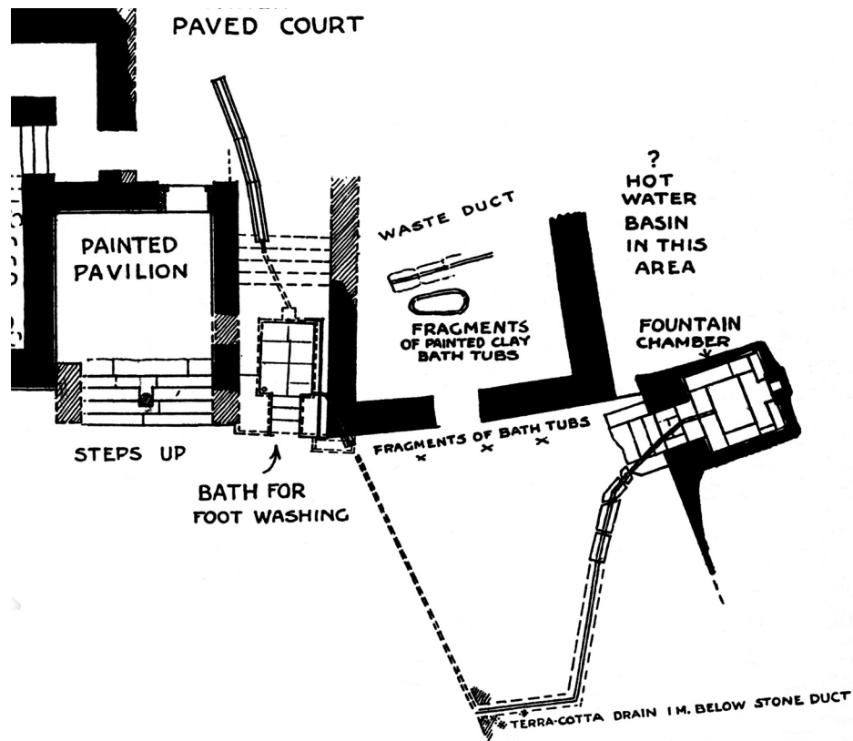
Fig. 8. Portion of Caravanserai area at Knossos (modified from Evans 1928, fig. 48).
