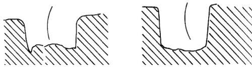
Fig. 1. Sections of three borings for mortises in the bathing slab at Tiryns (after Küpper 1996, fig. 104).
