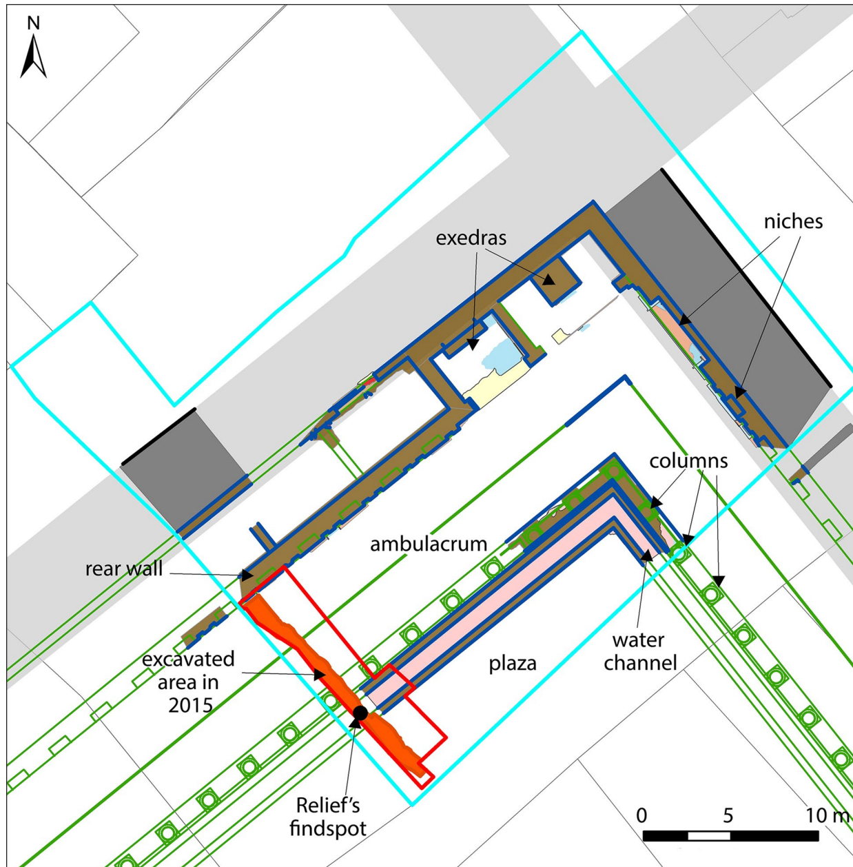
FIG. 3. Ground plan of the architectural structures open to the public in the Forum Portico (T. Barrientos).
