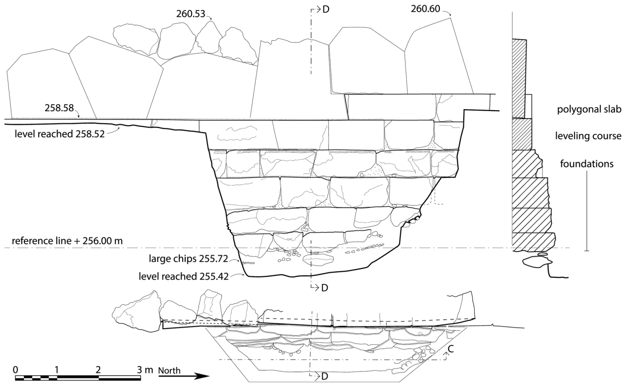
FIG. 14. Elevation ( top ), section ( right ), and plan ( bottom ) drawings of the sounding at the north end of the Late Archaic polygonal wall (drawings by G. Bianco).
