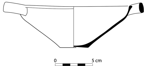
FIG. 8. Shallow angular bowl (P1878) from Tomb 12 in trench SWA1a west of the Blue Stone Structure (drawing by T. Ross).
